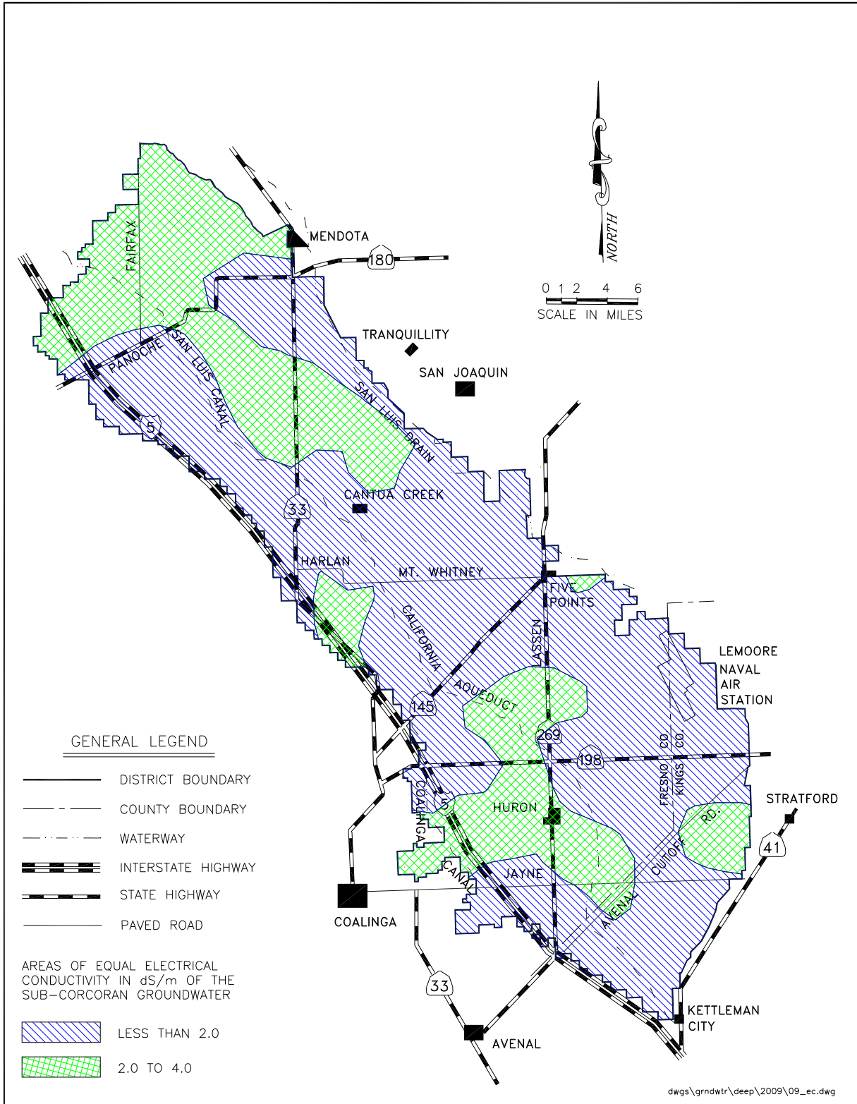
Figure 3: The Sub-Corcoran Groundwater, Electrical Conductivity (dS/m), December 2009.
