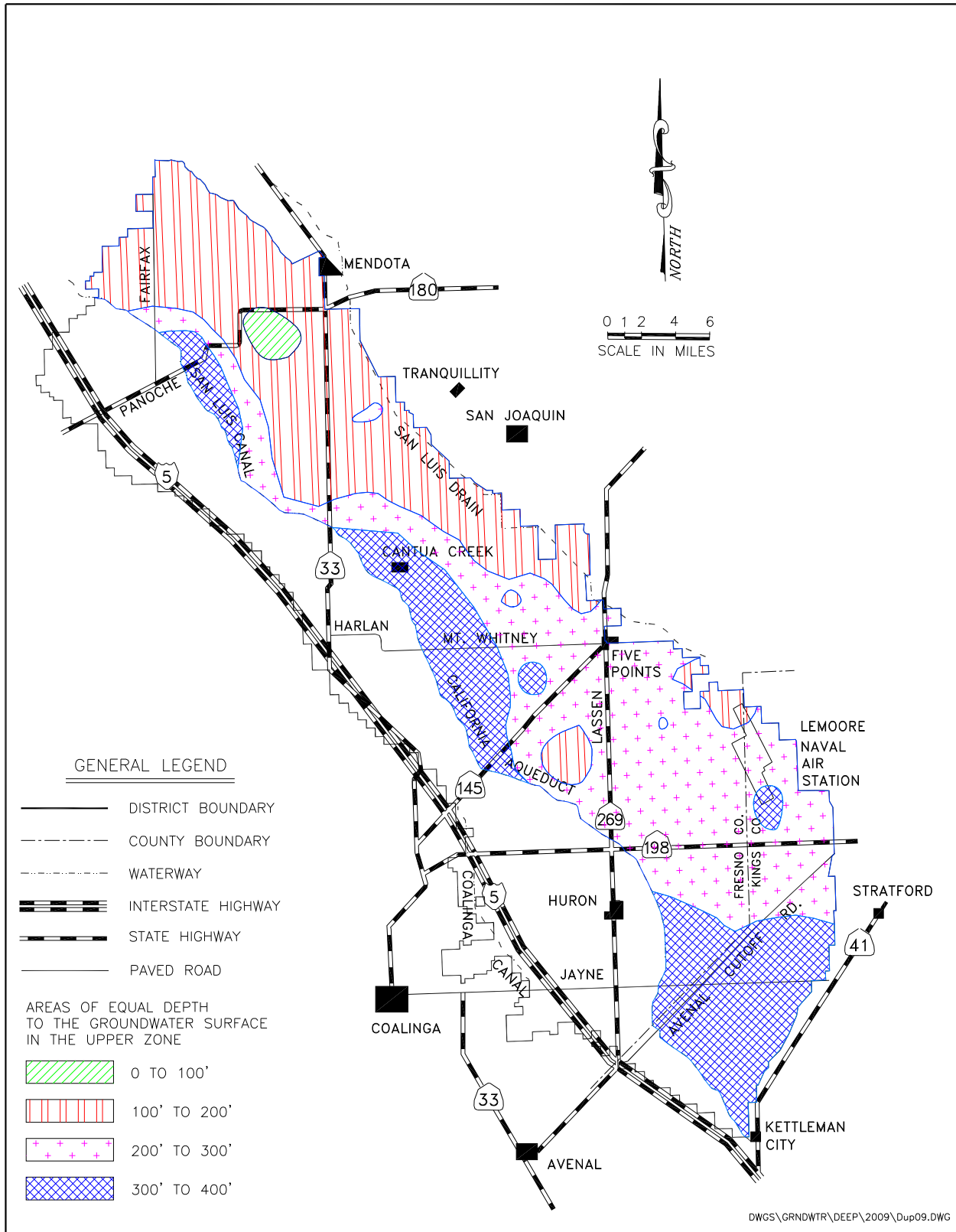
Figure 9: Depth to Groundwater in the Upper Zone, December 2009.
