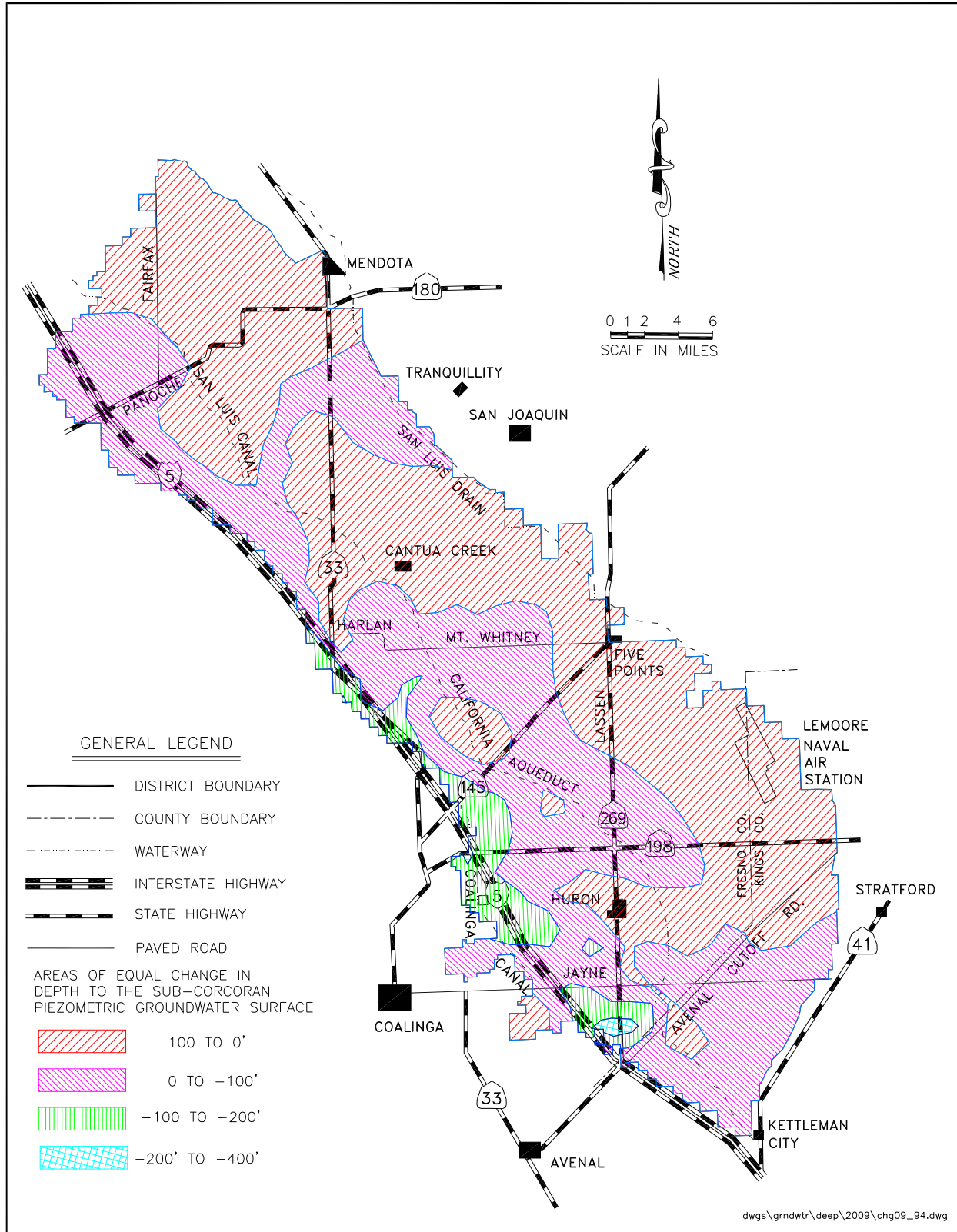
Figure 8: 1994 – 2009 Change in Depth to the Sub-Corcoran Piezometric Groundwater Surface.
