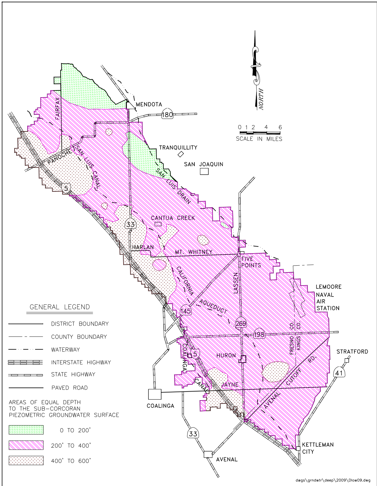
Figure 7: Depth to Sub-Corcoran Piezometric Groundwater Surface December 2009.
